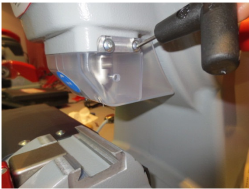
Loosen right side screws
