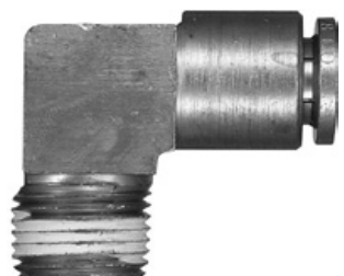
57512P Male Elbow 90° 3/8 Tube x 3/8 NPT
