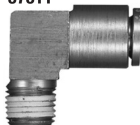
Male Elbow 90° 3/8 Tube x 1/4 NPT
