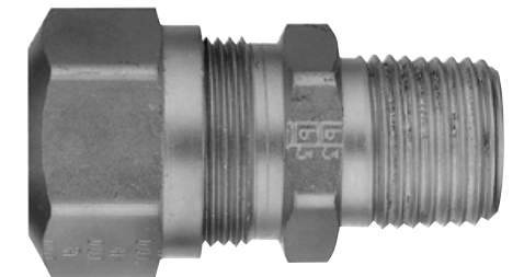
Male Connector 3/4 Tube x 1/2 Pipe
