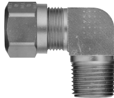
90° Male Elbow 5/8 Tube x 1/2 Pipe
